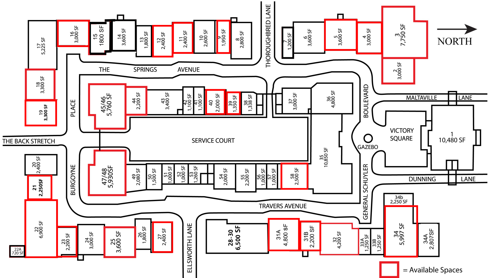
Site Plan
